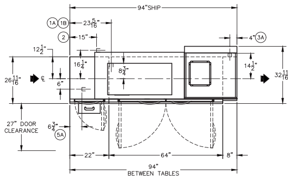
Plan View: Left to Right Model
