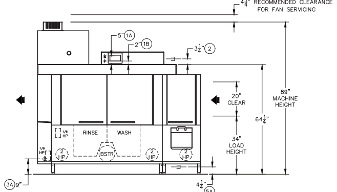
Front View: Right to Left Model
