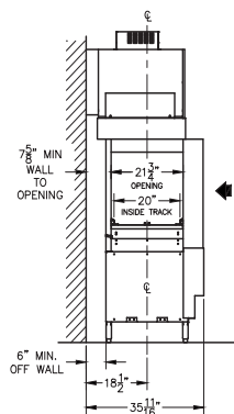
End View
