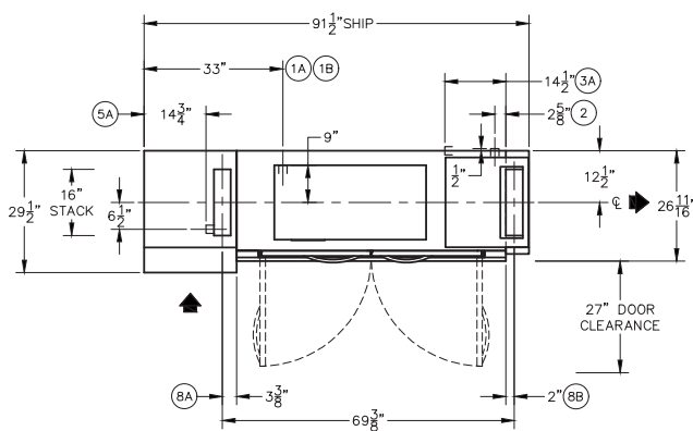
Plan View: Left to Right Model
