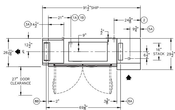
Plan View: Right to Left Model
