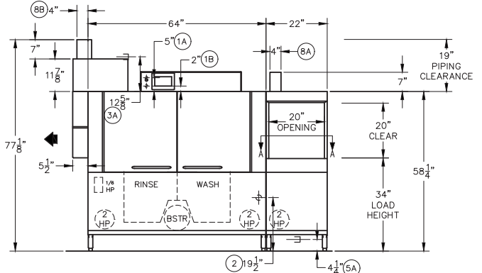
Front View: Right to Left Model
