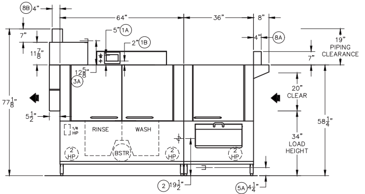
Front View: Right to Left Model
