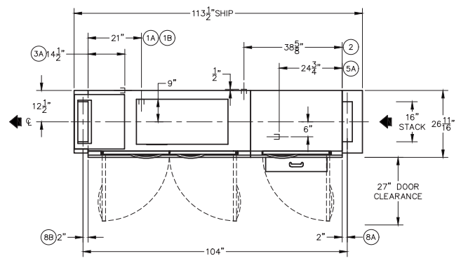
Plan View: Right to Left Model
