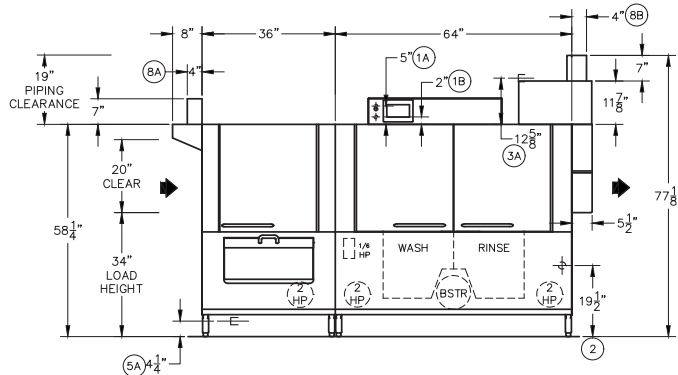
Front View: Left to Right Model
