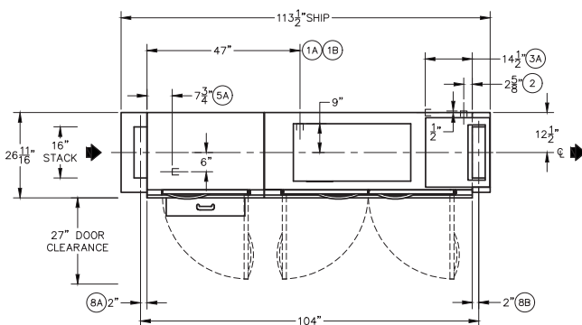
Plan View: Left to Right Model
